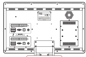
HDM08 Rear View
